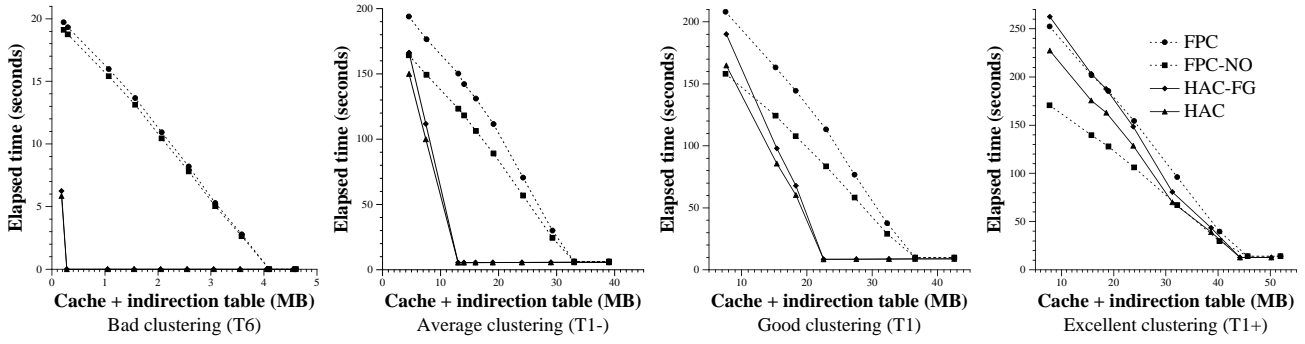
Figure 12: Elapsed time, Hot traversals, Medium database
